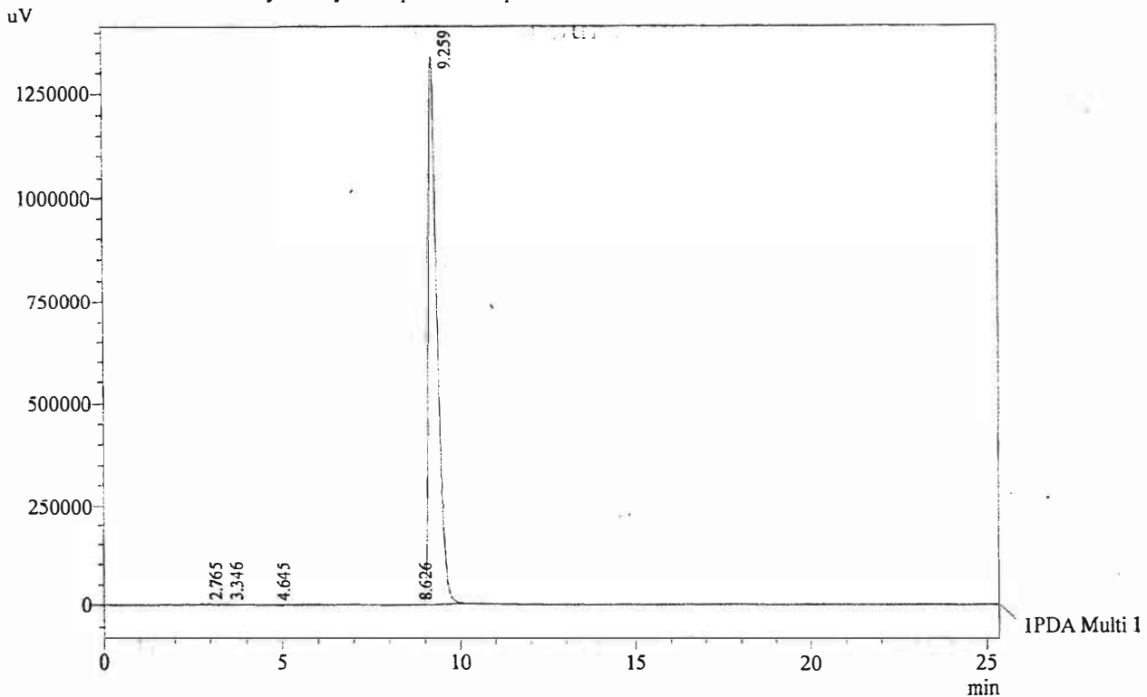
Chromatogram 4'-Cyclohexyl acetophenone D:\promonence\Data\2013JUNE-2013\170613J.lcd
